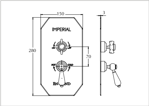
Concealed Cambridge thermostatic dual control valve (Edwardian chrome and Regent chrome lever controls)
