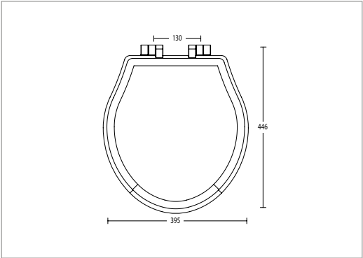
Regent painted toilet seat - with soft-close hinge Supplied without seat lid lift handle
