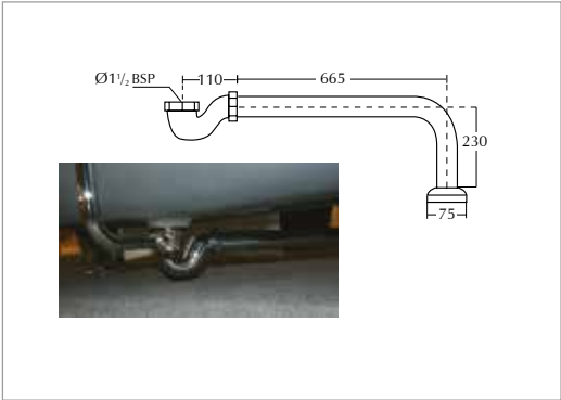
Roll top S trap low seal
