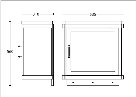
Carlyon cloak vanity basin (1 tap hole) White CR1MC11030
