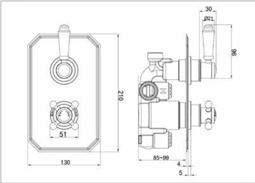
Concealed Lichfield thermostatic control valve (White controls) SINGLE WATER OUTLET
