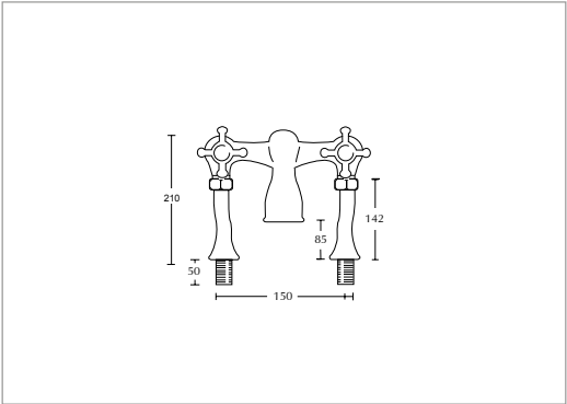
Bath filler, deck mounted (This bath filler has 150 centres)
