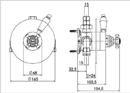
Concealed Westminster thermostatic control valve (White controls) SINGLE WATER OUTLET
