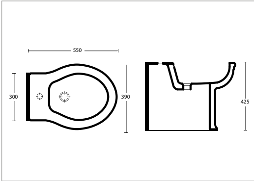
Back to wall bidet (1 tap hole) White RG1BB11030
