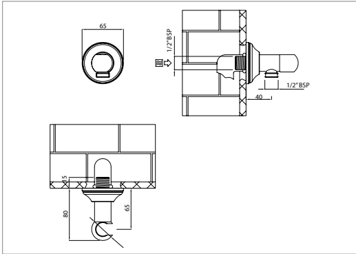
Hand shower kit (Suppled with either a white or black handset) For use with the concealed shower valve
