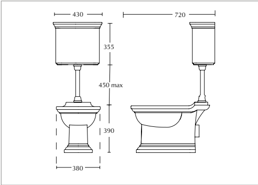
A) Low level cistern - Ceramic plate option (including all the components) fittings White/Chrome ZRDLC01000C White/Antique Gold ZRDLC01000I White/Polished Nickel ZRDLC01000N White/Brushed Nickel ZRDLC01000BN White/Brushed Brass ZRDLC01000BB
