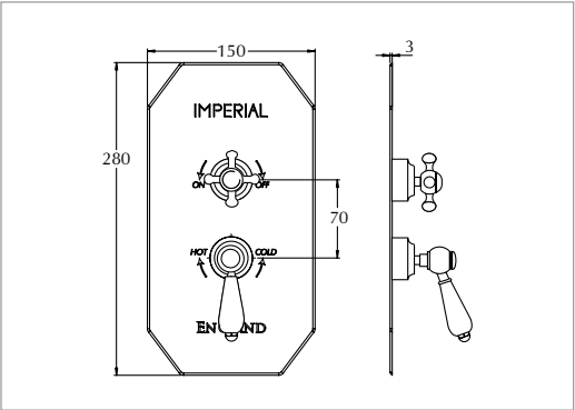
Concealed Cambridge thermostatic dual control valve (Victorian white and Radcliffe white lever controls)
