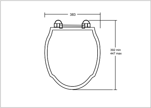
Westminster solid wood toilet seat - with soft-close hinge Supplied with seat lid lift handle in the box
