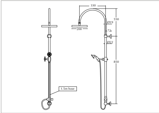
Edwardian rigid riser - slim Amena shower head* (White handset)
