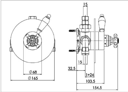
Concealed Westminster thermostatic control valve (Black controls) SINGLE WATER OUTLET
