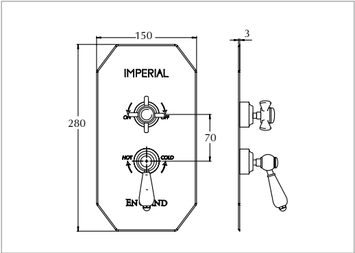
Concealed Cambridge thermostatic dual control valve (Edwardian Black and Radcliffe Black lever controls)
