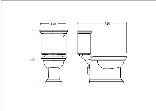
A) Radcliffe close coupled cistern Lever Option fittings White/Chrome ZRDCC01000C White/Antique Gold ZRDCC01000I White/Polished Nickel ZRDCC01000N White/Brushed Nickel ZRDCC01000BN White/Brushed Brass ZRDCC01000BB
