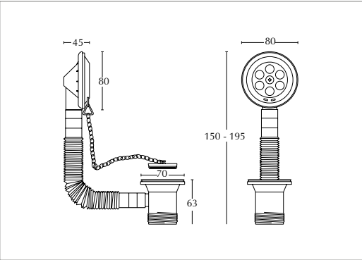
Tidy plug standard bath waste with plug and chain
