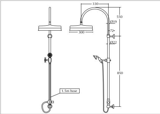
Edwardian rigid riser - traditional Lichfield head* (White handset)
