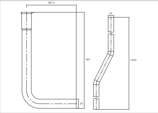
High level flush pipe* For Lichfield, Drift, Oxford, Etoile, Chelsea and Heyford
