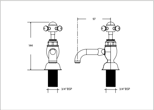
3/4" bath pillar taps
