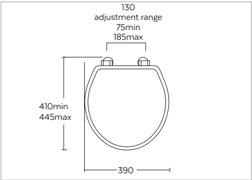
Windsor painted toilet seat - with soft-close hinge Supplied without seat lid lift handle
