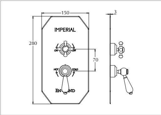
Concealed Cambridge thermostatic dual control valve (Victorian Black and Radcliffe Black lever controls)
