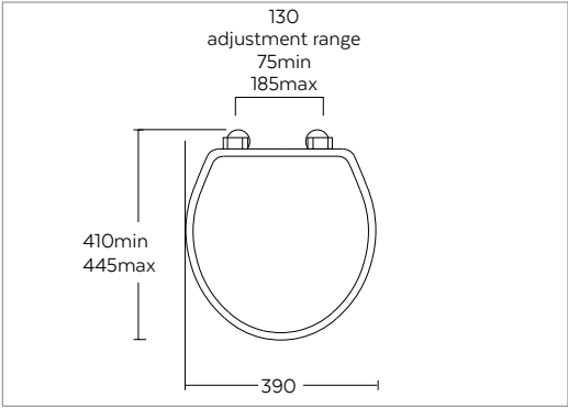
Windsor solid wood toilet seat - with soft-close hinge Supplied with seat lid lift handle in the box
