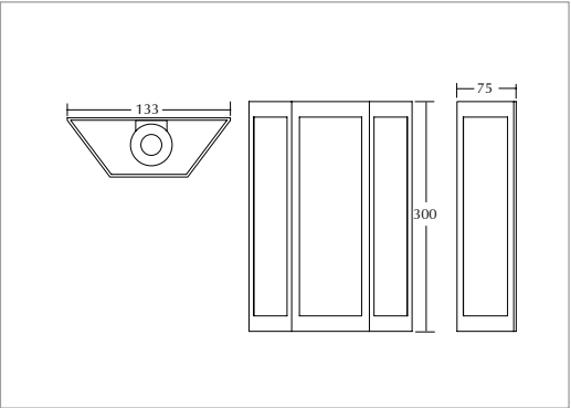
Empire wall light
