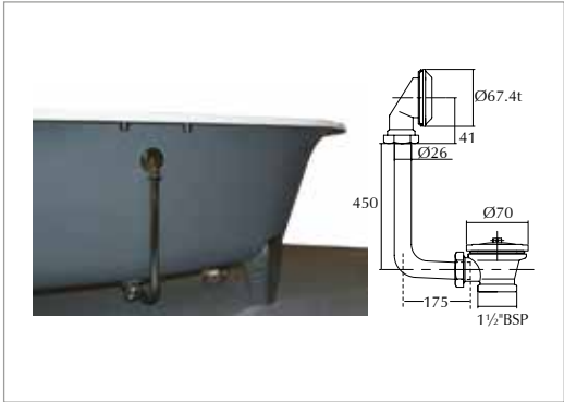
Exposed bath waste
