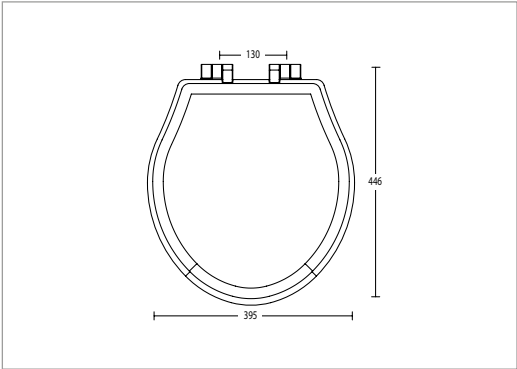
Regent solid wood toilet seat - with soft-close hinge Supplied with seat lid lift handle in the box
