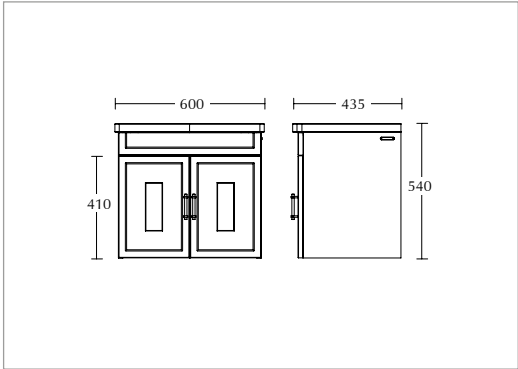
Radcliffe medium vanity basin (1 tap hole) White RD1MI11030N (3 tap hole) White RD1MI31030N
