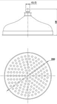
Lichfield traditional Shower Head 200mm (supplied without the round wall arm)
