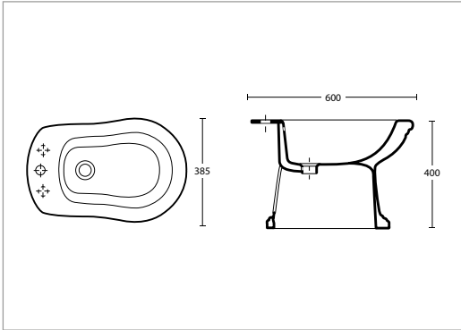
Free standing bidet (1 tap hole) White RG1BI11030
