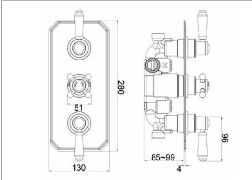
Concealed Lichfield thermostatic dual control valve (White controls) TWIN WATER OUTLET
