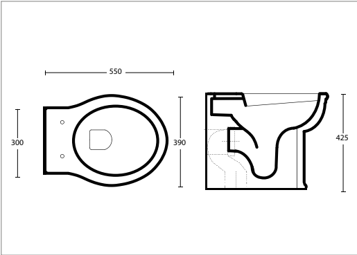
Back to wall pan (supplied without cistern fittings) (For use with Regent seat) White RG1BC01030
