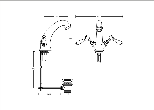
Tall mono basin mixer (complete with pop up waste)
