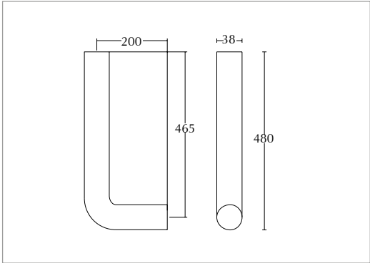
Low level flush pipe & shroud For Lichfield, Drift, Oxford, Etoile, Chelsea and Heyford
