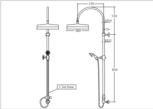
Edwardian rigid riser - traditional Lichfield Rose (White handset) For use with the concealed shower valve
