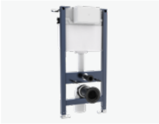
Wall Hung 0.98m Support Toilet Frame Dual flush concealed cistern and installation kit included W: 450 L: 159 H: 980 Code: BR_WCF98X45R
